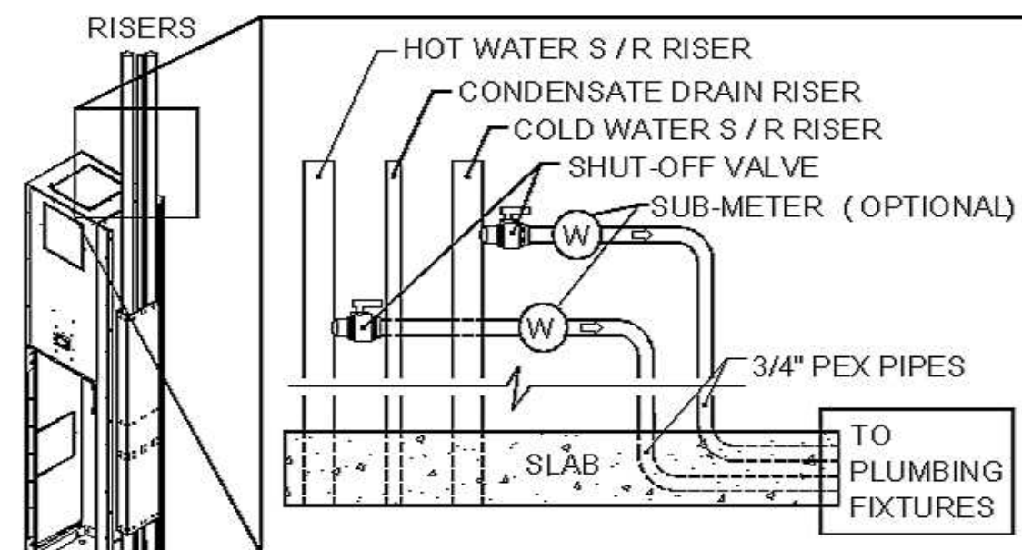
IPS FAN COIL WITH PEX TUBING INSTALLTION IN CONCRETE APPLICATION.
