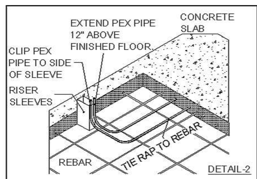
IPS FAN COIL WITH PEX TUBING INSTALLTION IN CONCRETE APPLICATION.
