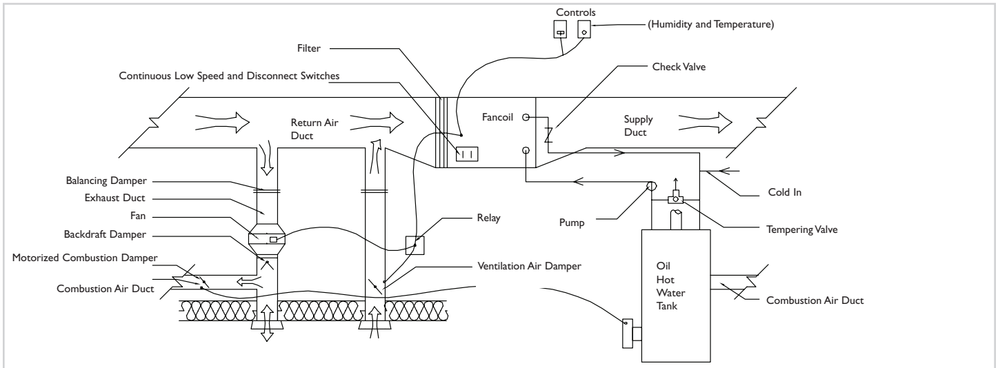
Figure 1 High velocity fancoil integrated combination heat, ventilation and domestic hot water system
