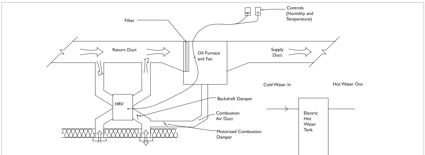
Figure 2 Heat Recovery Ventilation (HRV) with Forced Air Furnace
